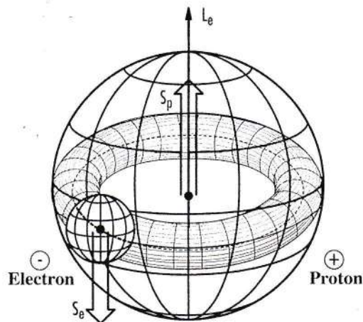
FIG. 6. Image of the hydrogen atom's electron orbiting within the proton forming a neutron in
