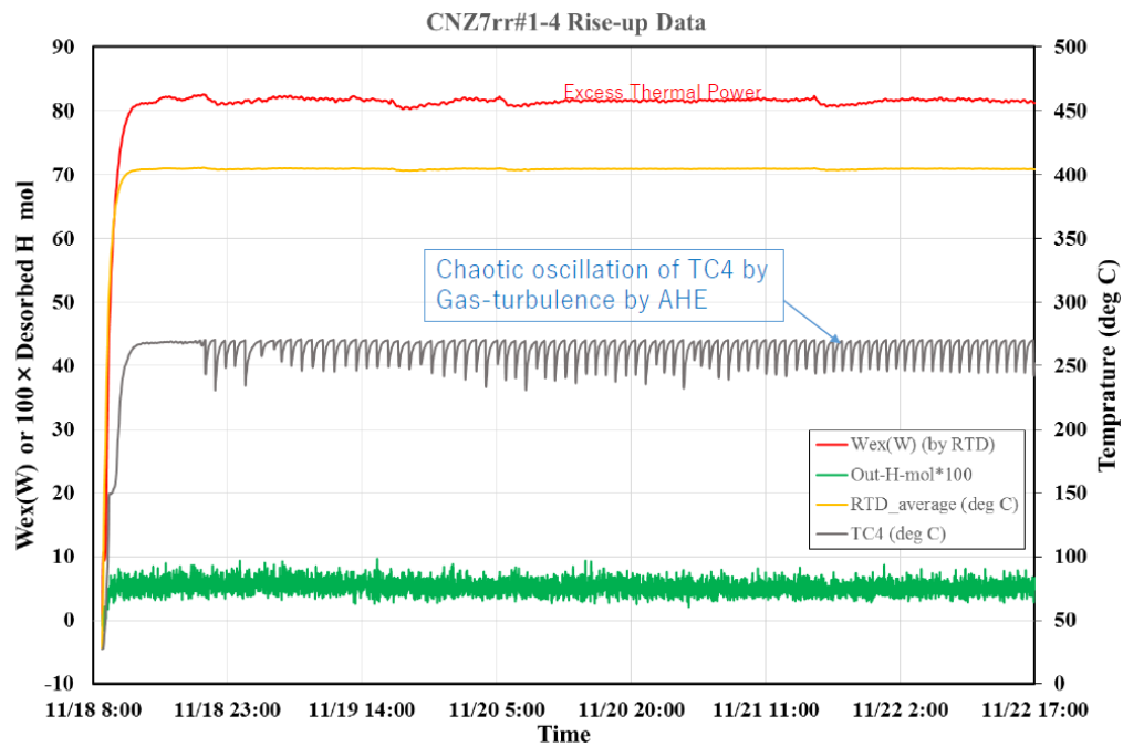
FIG.13; 5; 5; 5 days long run of CNZ7rr #1-4 with [140, 95] W heating
