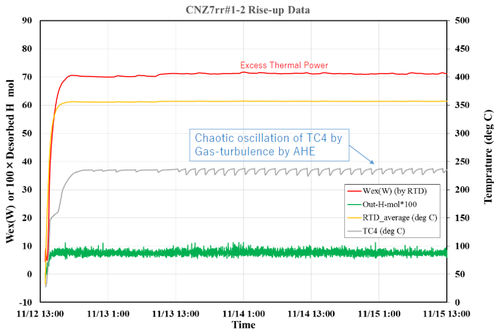
Fig.12; One week-days data of AHE by CNZ7rr #1-2-2 run
