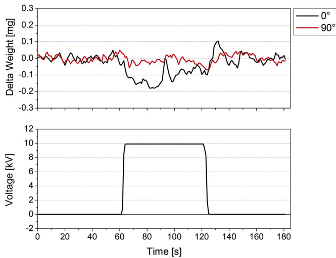
Fig. 8. Weight change of asymmetric Teflon capacitor.
