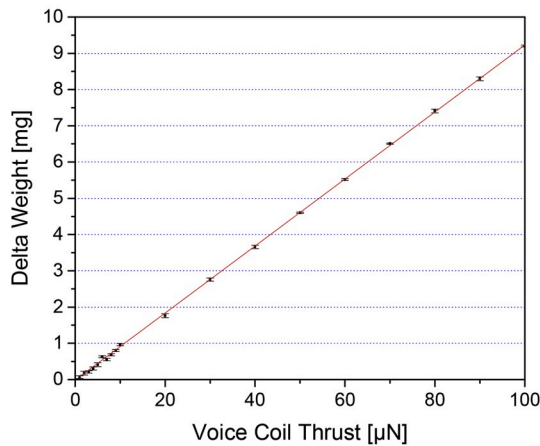
b) Balance Linearity
