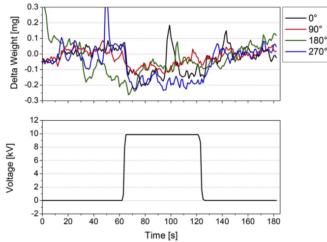
Fig. 5. Weight change of high voltage ceramic capacitor.
