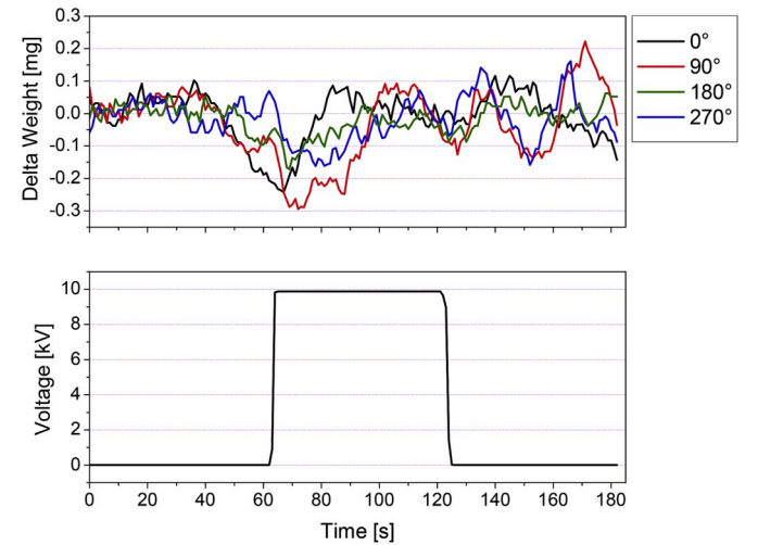
Fig. 7. Weight change of symmetric Teflon capacitor.
