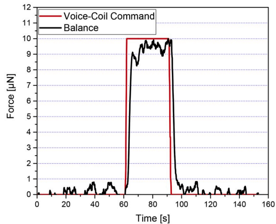
c) Balance Response at 10 \mu\text{N} (=1 mg)
