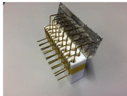
e) Liquid-Metal Connection Pins
