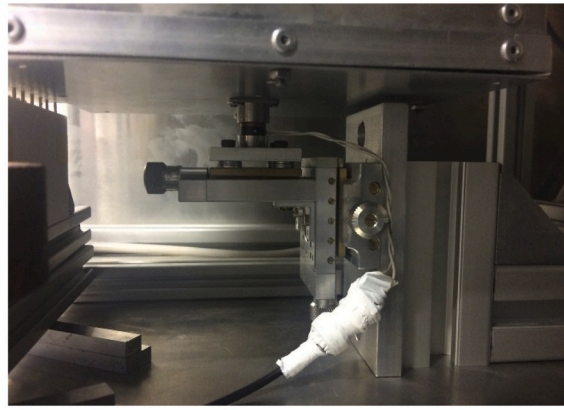
a) Voice-Coil below Experiment Box
