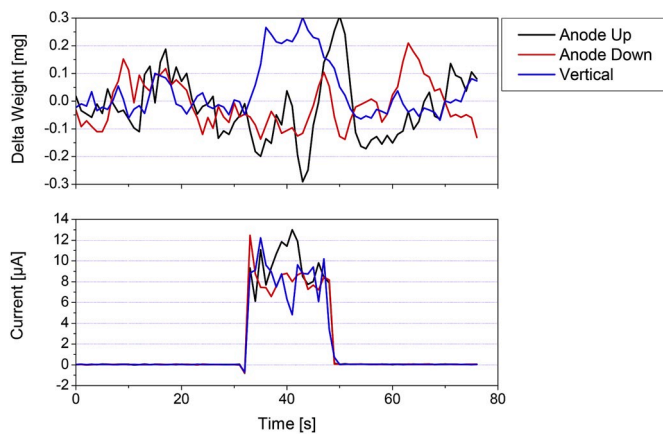
Fig. 12. Weight change of leakage capacitor at 2100 V.
