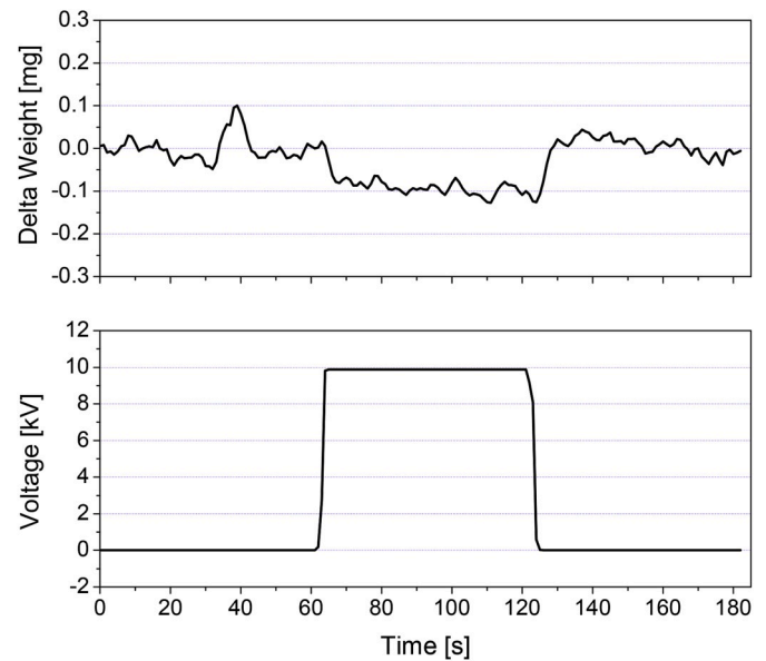
Fig. 10. Weight change of spherical capacitor.
