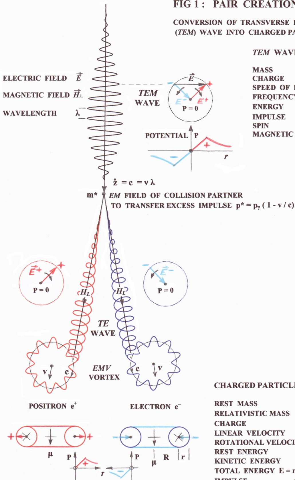
FIG 1: PAIR CREATION CONCEPT
