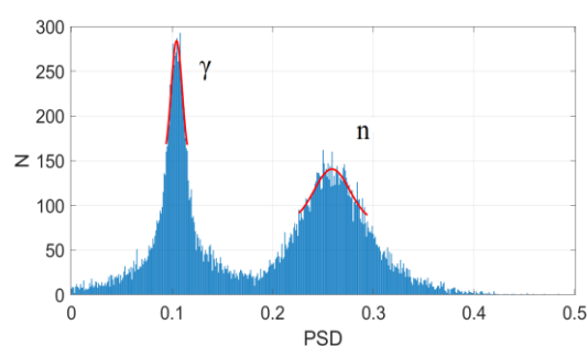
Figure 2. PSD histogram with fitted top of each peak with a Gaussian curve.
