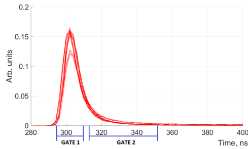
Figure 3. Oscilloscope of a group of normalized signals.
