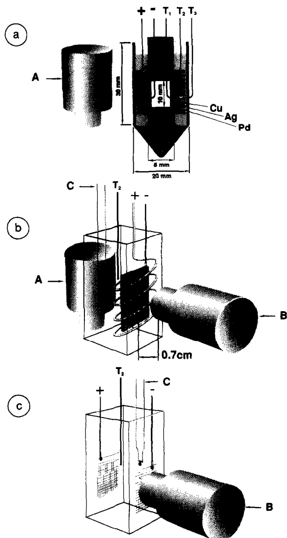
Fig. 2. Electrolytic cells. (A) \gamma -ray detector; (B) X-ray detector; (C) reference electrode; thermocouples: T_1 attached to the interior of the working electrode; T_2 immersed in the electrolyte; T_3 to measure the cell wall temperature. (a) Centrally located electrodes assembly; cell designed for examination of the spectral region 15–3000 keV. (b) Movable electrode assembly; closest approach of the working electrode to the detector window of 0.5 cm; cell designed for the spectral region 15–300 keV and provided with dual detection system. (c) Cell designed for detection of soft X-rays. The detector window is separated from the working electrode by the thickness of the Mylar sheet.
