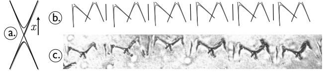
FIG. 36. a.) Intersection of tachyon with plane parallel to particle motion on x axis. b.) Simulation of “M” components of track with periodic structure using conic sections. c.) Track from Fig. 4 exhibiting periodic structure.
