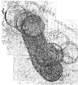
FIG. 20. Matsumoto correlated tracks overlaid. The shape of the image and certain ring positions correspond.
