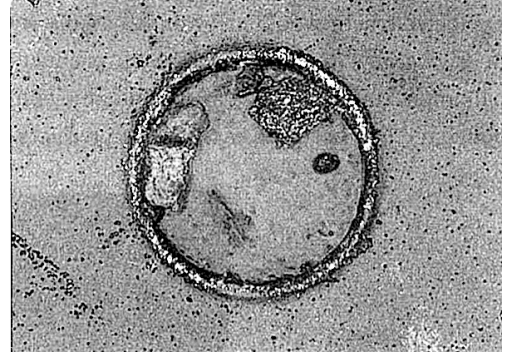
FIG. 35. Ring track of Matsumoto
