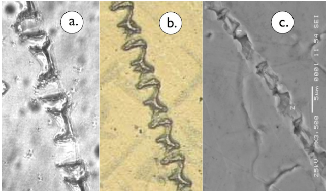
FIG. 3. a.) Fredericks track on Polychrome litho film. b.) Rodinov and Savvatimova periodic structure track on nuclear emulsion. Note similarity to Fredericks track where "hour-glass" structures are separated by flat structures. c.) Rodinov and Savvatimova periodic structure track on Pd cathode from scanning electron microscope.
