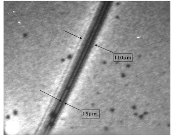
FIG. 25. Sub Tracks Detail Micrograph at 45x magnification showing sub-track structure of the track bundle.
