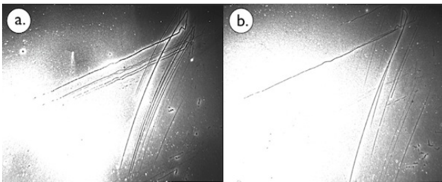
FIG. 21. bobby pins raw tracks in Kodak NTB3 10 \mu emulsion. Tracks a and b are separated by a few millimeters on the film. Tracks have many of the same features, except that track a has a loop, i.e. the track crosses itself whereas track b does not. These tracks are correlated in position extremely well until the critical region (segment 19 in Fig. 22.) when track a has a large angle deflection to the left and track b has a corresponding smoothly curving deflection to the right. Susceptibility to magnetic deflection appears to be overwhelming or twisting the correlation.
