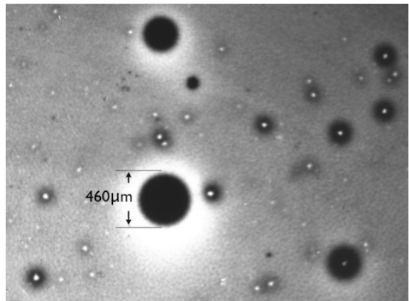
FIG. 9. Micrograph at 25x of dots. Note the internal structure of all-black dots and dots with white centers. Kodak type NTB3 10\text{ }\mu emulsion.
