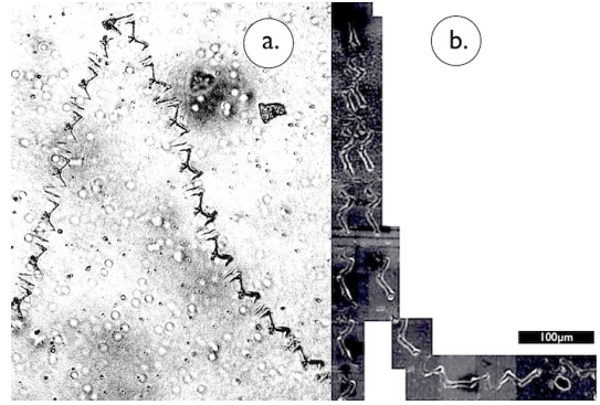
FIG. 4. a.) Fredericks track b.) Adamenko and Vysotskii track evaporated in MDS showing parabolic curvature. Detail of track using high magnification.
