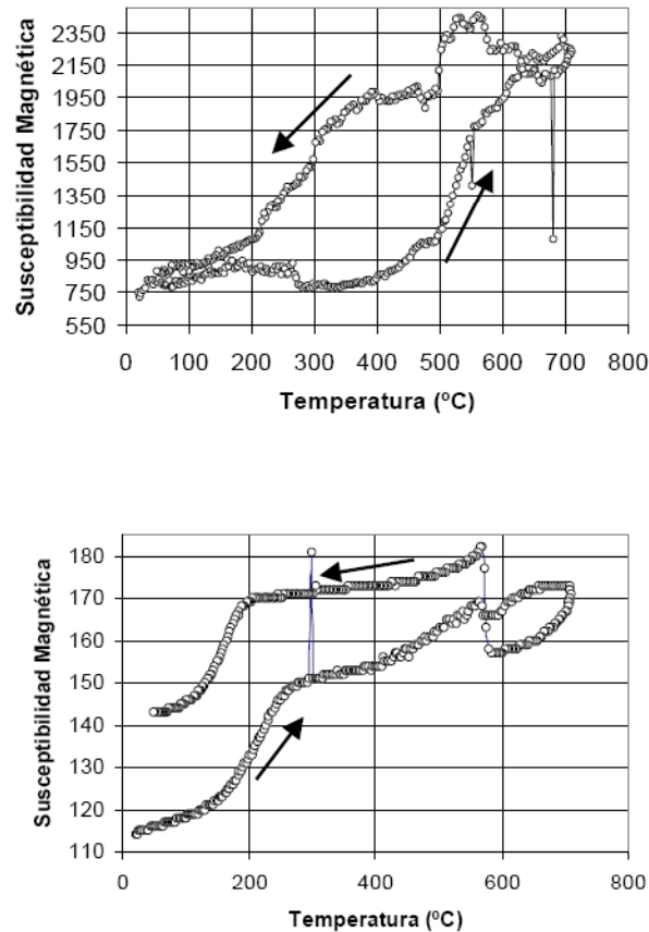
Figure 11. Behavior of two surface samples of the Veas-01 rock. Magnetic susceptibility was not lost even beyond the upper limit of the heating oven at approximately 760°C. Figure 11a at top, 11b at bottom.
