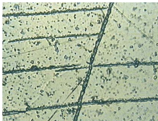
Figure 13. Metallurgical microphotograph of a metallic sample of the Veas-01 rock, at 500x (IDIEM). Neumann Lines are revealed, a common feature to siderites.
