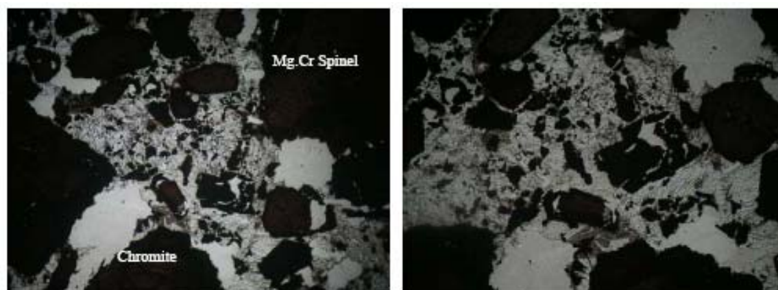
Figure 2. Micropetrographic photographs of sample Oliv02. a) Chromite and Mg,Cr spinel (up to 7 mm) in a monticellite – melilite (?) – leucite matrix. b) detail of matrix.
