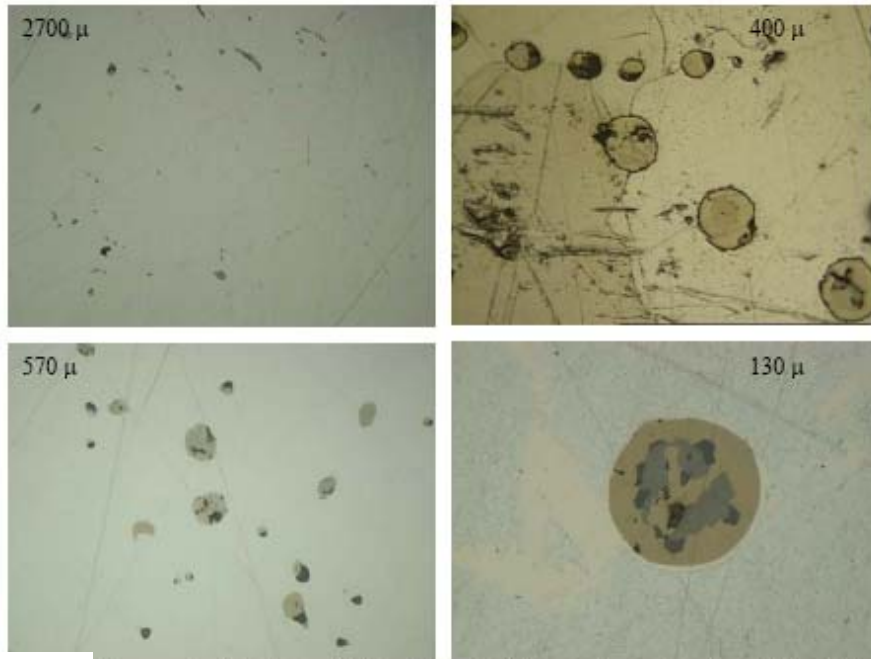
Figure 6. a) iron sample with inclusions (2700 \mu side wize), Widmannstaetten texture pattern slightly visible, hexagonal habit of crystals; b) iron sample with inclusions (400 \mu side wize), hexagonal contacts between crystals; c) iron sample with inclusions (570 \mu side wize); d) detail of inclusions (130 \mu side wize).
