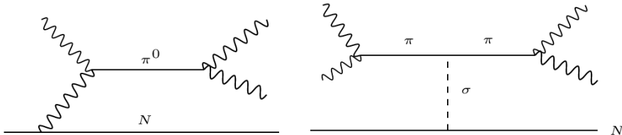
Figure 2: Left: Primakoff effect. Right: Instead of having a photon from the nucleon a \sigma meson is between the nucleon and the photons. Here with pions inbetween even if direct photon \sigma interaction exist.
