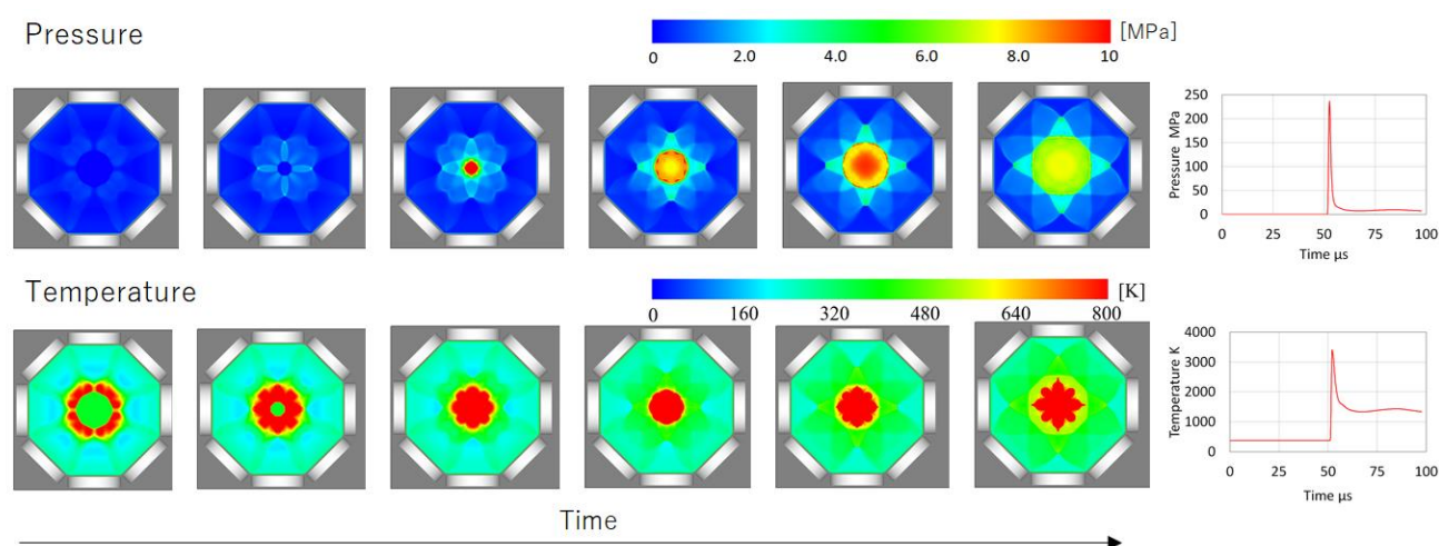
Fig. 1 Computational results of single focusing collision of 26-pulsed supermulti-jets with high speed. Spatial distribution of pressure and temperature, and time history of pressure and temperature at the collision point.
