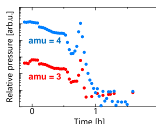
Fig. 3 Pressure evolution.
