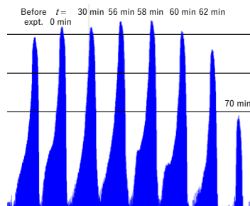
Fig. 2 Mass spectra for amu = 4.
