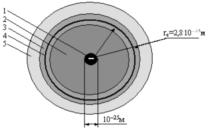
Fig.16. The structure of an electron in a vacuum field.
