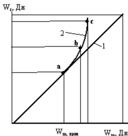
Fig.5. Nonlinear dependence of mechanical work and thermal energy.
