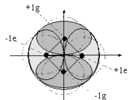
Fig.11. The formation of the quanton as a compression of monopoles into a single quantum.
